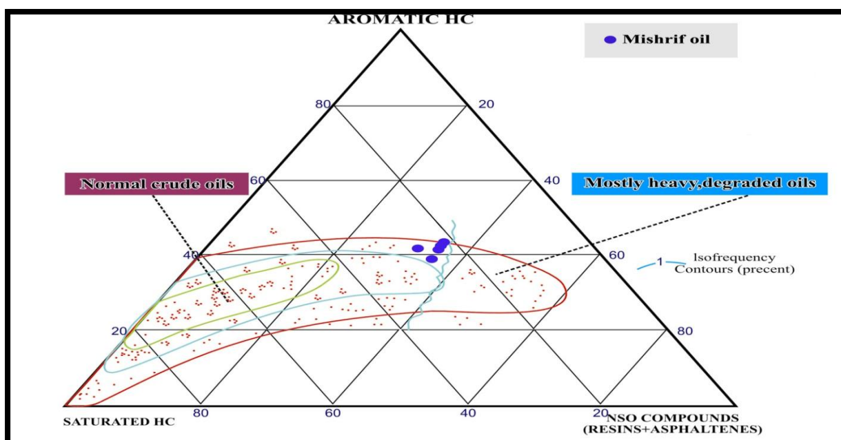
Figure 6- Ternary diagram showing the gross composition: saturated hydrocarbons, aromatic hydrocarbons, and resins plus asphaltenes for crude oil samples of Noor oilfield
