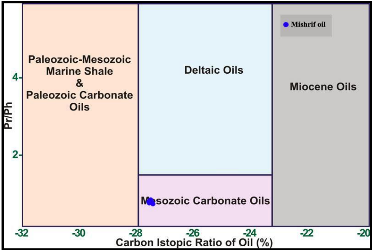
Figure 4- Relationship between pristane/phytane and Carbon isotopic ratio of oil (%) for crude oil samples of Noor oilfield to predicate source rock environment and age
