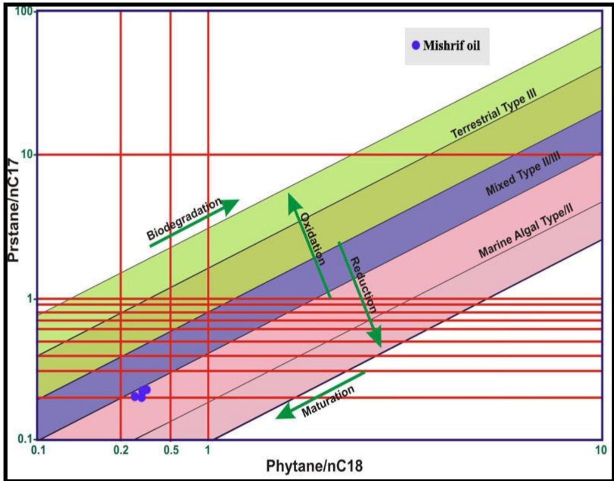
Figure 3- Shows cross plot between pristane/nC17 versus phytane/nC18 for Mishrif crude oil
