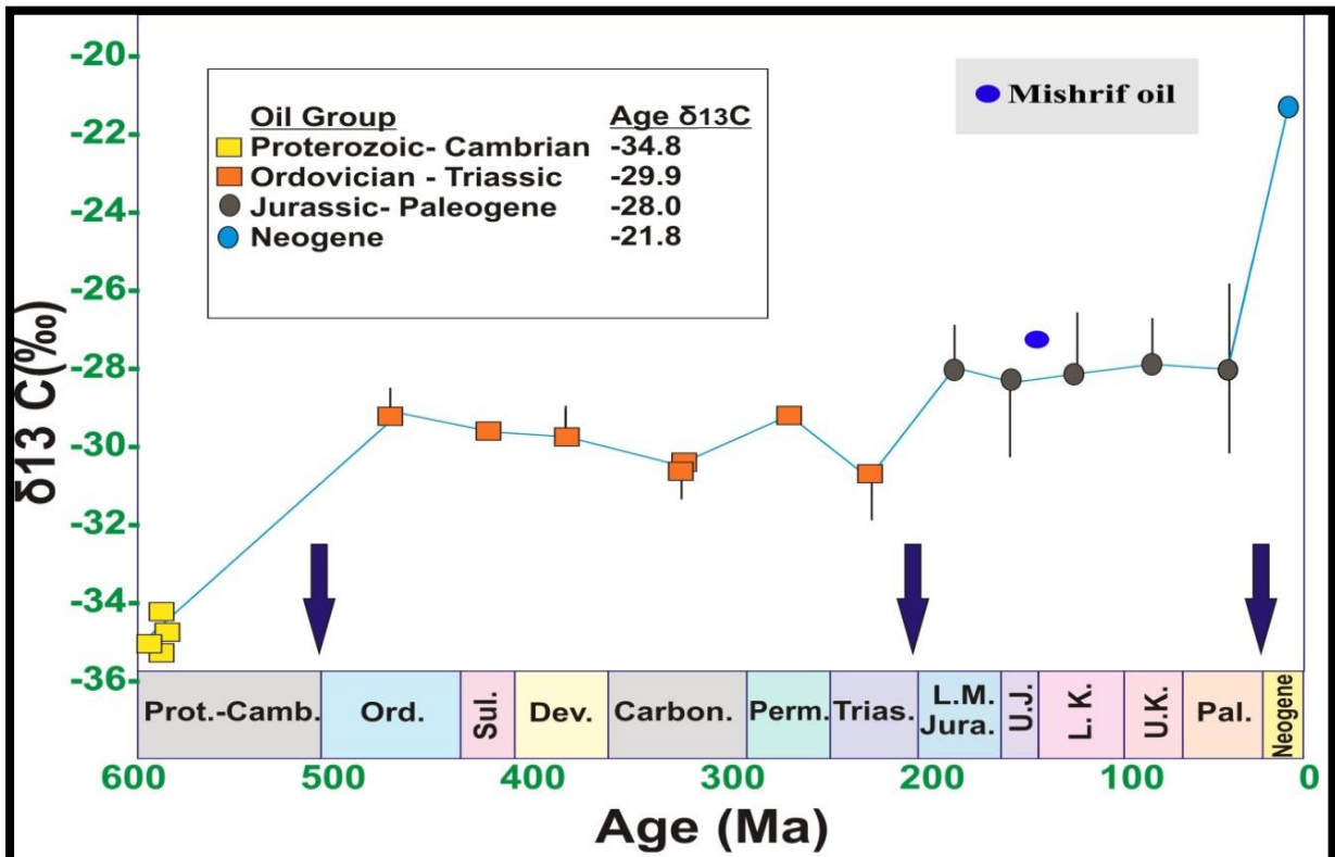
Figure 5- Average stable carbon isotopic ratios for C15+ saturated fractions oil versus age for crude oil samples of Noor oilfield
