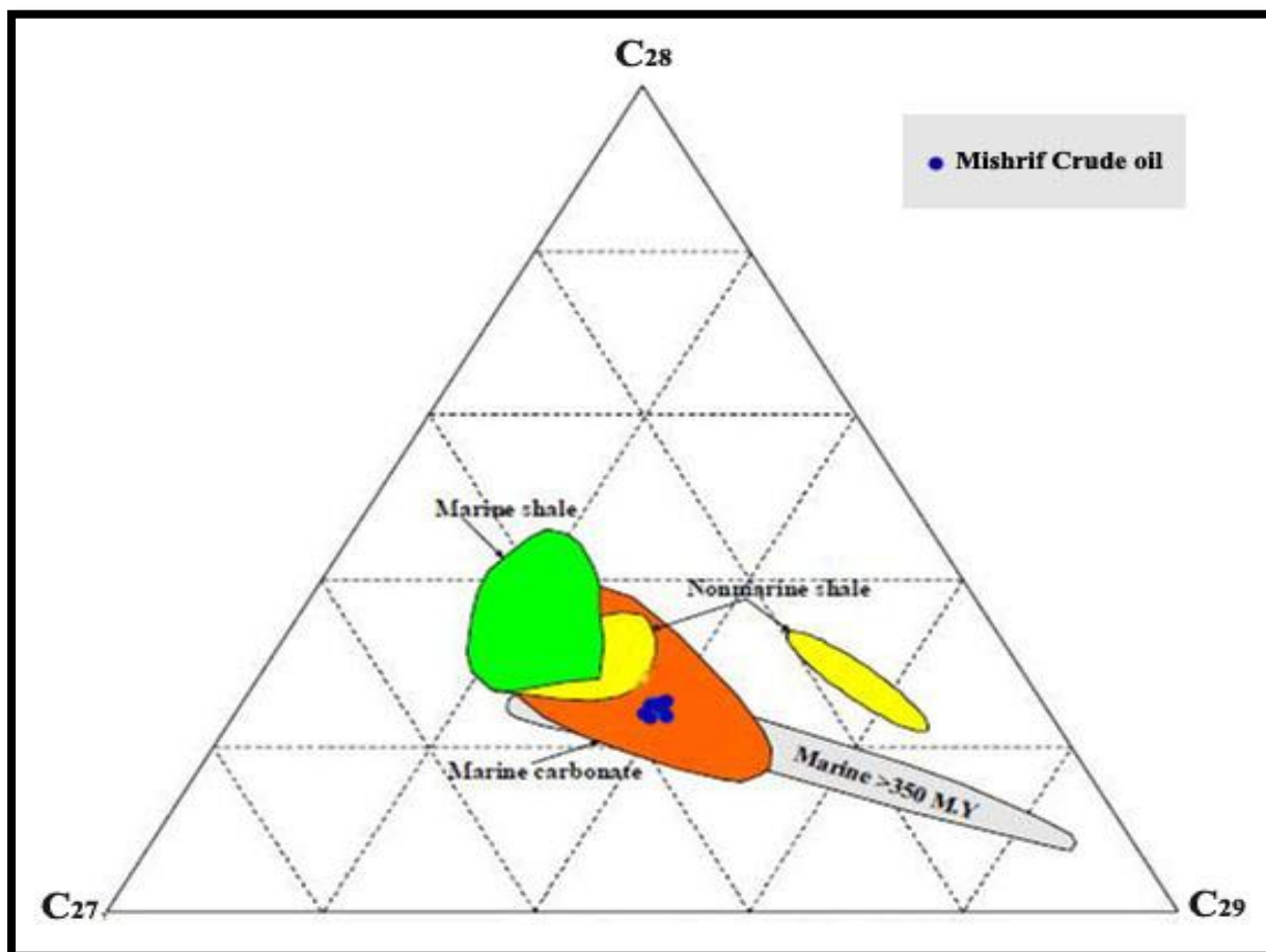
Figure 2- Ternary diagram showing the relative abundances of C27, C28, and C29 regular steranes of Mishrif crude oil
