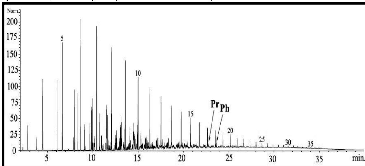
Figure 7- Whole crude chromatograms for No-1 oil sample
